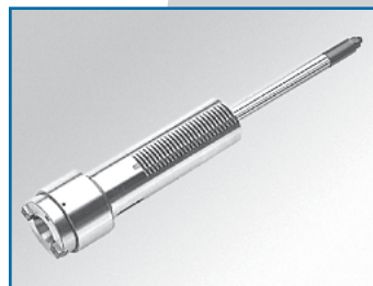
CODE 40020: Asse mandrino ISO 40 con tirante (DIN 2080) ISO 40 spindle including tie-rod (DIN 2080)
